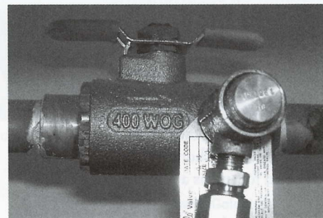
Photo 2: A thermal expansion valve
